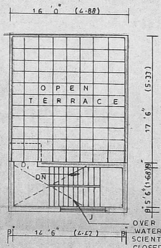
OPEN TERRACE PLAN
